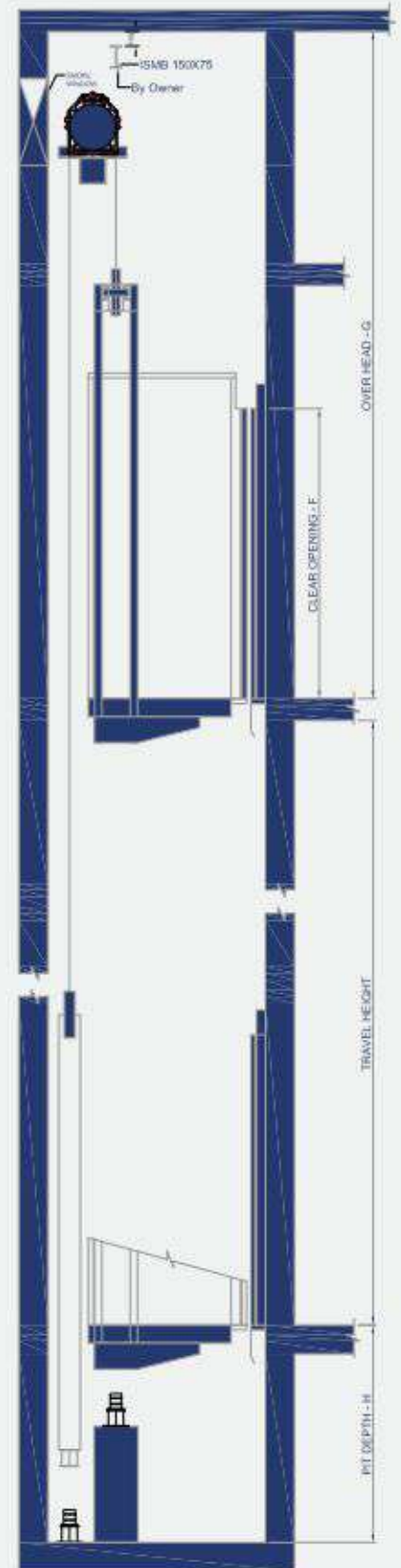
HOISTWAY SECTION
