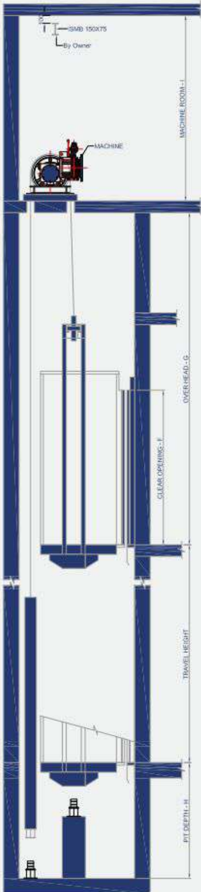
HOISTWAY SECTION
